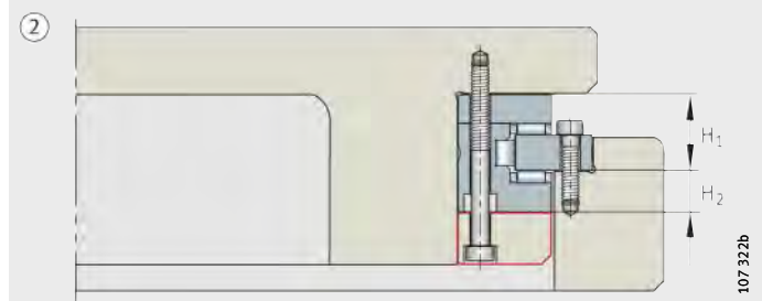
Figure 17 Mounting variants
